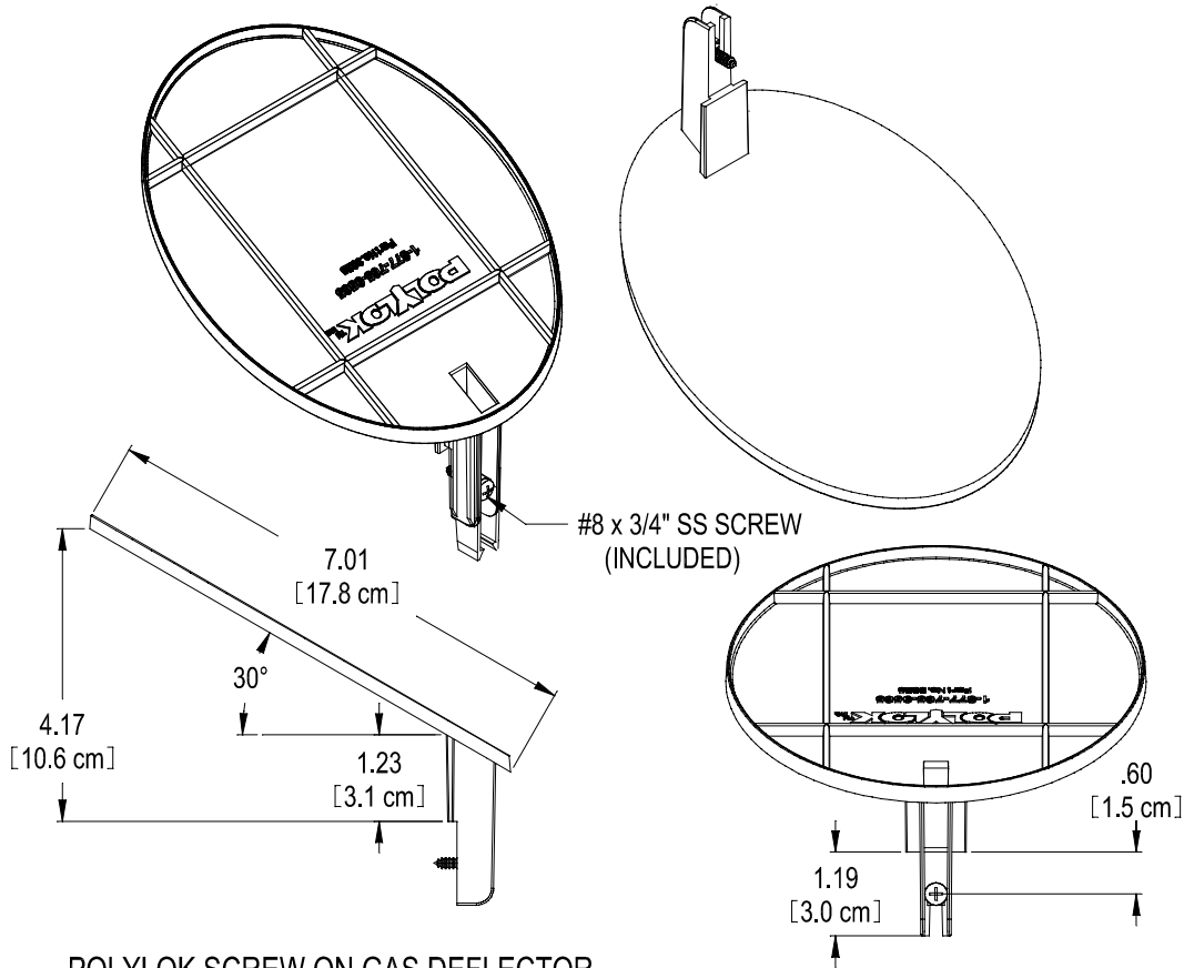
POLYLOK SCREW ON GAS DEFLECTOR PART NO. 3025-S MATERIAL - POLYPROPYLENE COLOR - BLUE
